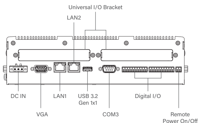
Rear I/O
